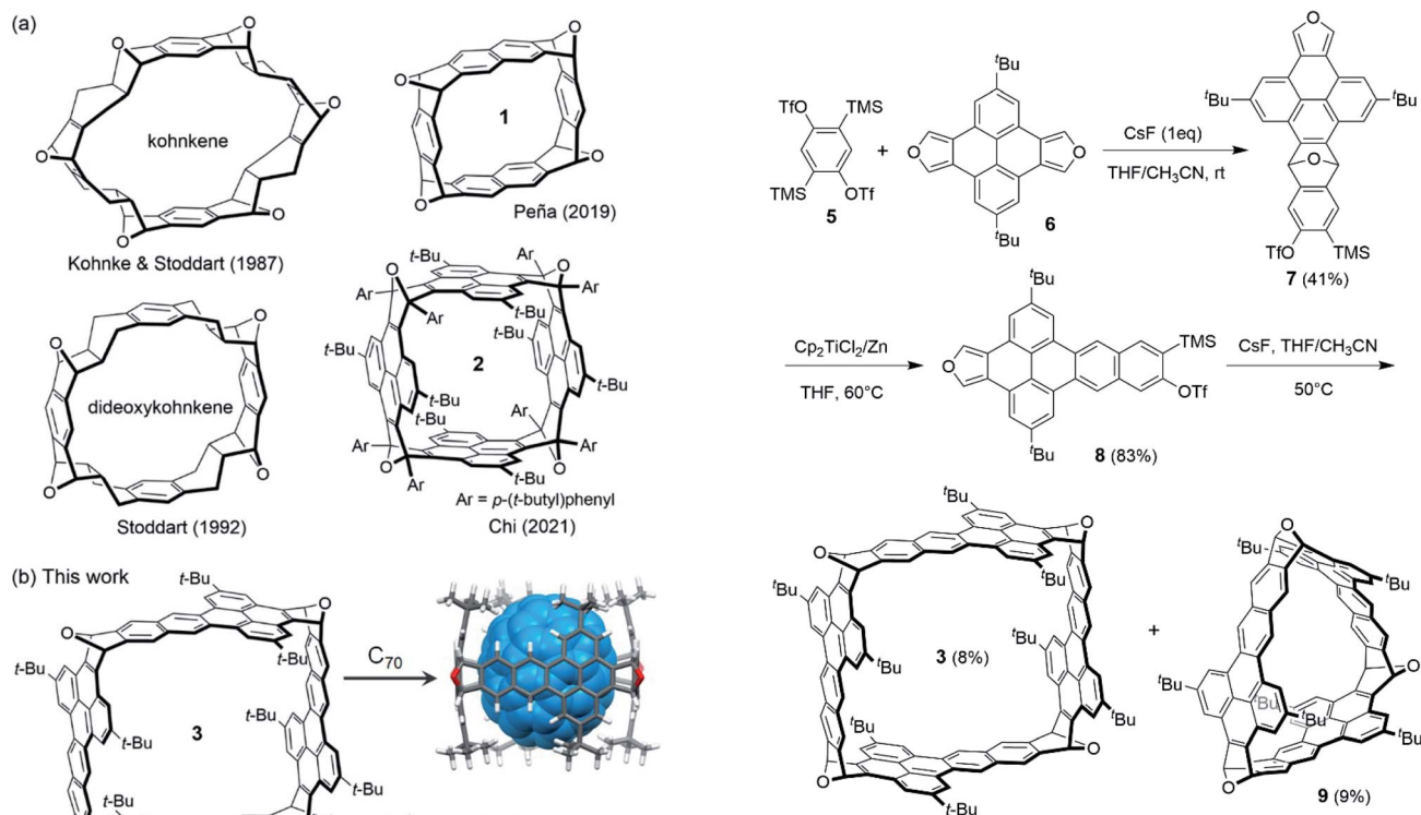
Scheme 1 Synthesis of 3.
