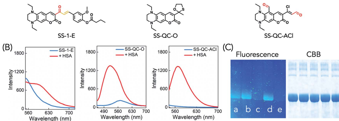
Fig. 2 Covalent binding site verification of HSA and SS-1. (A) Reaction site based modification of the fluorescent dyes. (B) Fluorescence responses of 5 \mu\text{M} SS-1-E, SS-QC-O and SS-QC-ACI toward HSA (2 \text{mg mL}^{-1} for SS-1-E, 0.5 \text{mg mL}^{-1} for SS-QC-O and SS-QC-ACI) in PBS, respectively. SS-1-E: \lambda_{\text{ex}} = 516 , slit 5/5 nm, 700 V; SS-QC-O: \lambda_{\text{ex}} = 440 , slit 2.5/5 nm, 700 V; SS-QC-ACI: \lambda_{\text{ex}} = 505 , slit 2.5/5 nm, 700 V. (C) Covalent labeling verification of HSA by SS-1, SS-1-E, SS-QC-O or SS-QC-ACI analyzed by SDS-PAGE gel. (a–d) Represent the addition of the four fluorescent dyes (40 \mu\text{M} ) to HSA (1.25 \text{mg mL}^{-1} ), respectively; (e) is the control group without dye addition.
