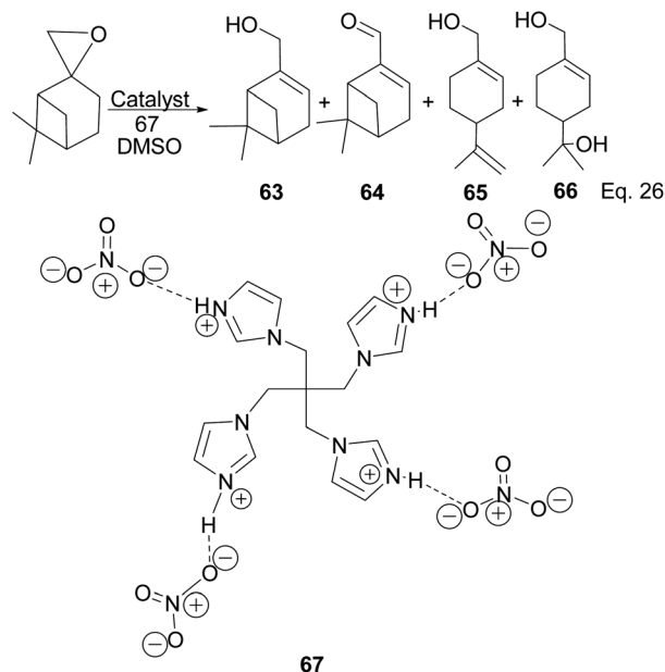
Scheme 22 Myrtenol, myrtenal, and terpineol derivatives of \beta -pinene oxide.
