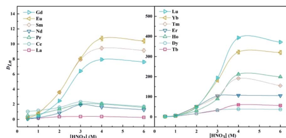
Fig. 3 Effect of HNO 3 on the extraction of Ln(III) by L II in 40/60 (v/v)% n -octanol/kerosene (O : A = 1 : 1, [Ln^{3+}]_{init} = 3 mM).
