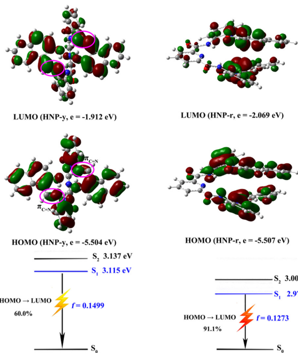
Fig. 5 The frontier orbitals and theoretically calculated vertical excitation energies, transition natures of the excited states and oscillator strengths for HNP-y and HNP-r .
