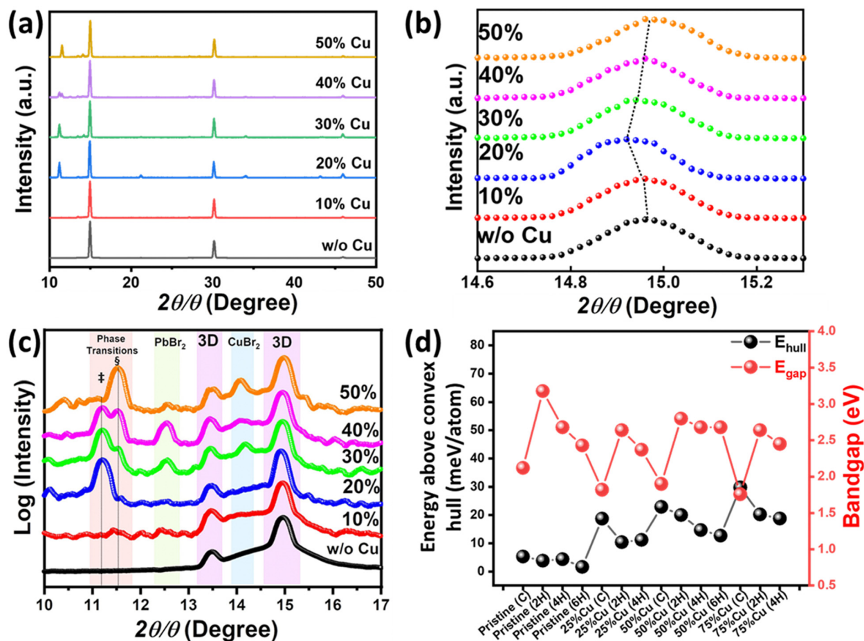
Fig. 3 (a) XRD patterns of Cu-alloyed MAPbBr 3 perovskite thin films. (b) XRD peak (100) shift upon copper addition. (c) XRD patterns (log scale) for 2\theta = 10-17^\circ . (d) Energy above convex hull and bandgap for different phases of pure and Cu-alloyed MAPbBr 3 where C, 2H, 4H, and 6H represent cubic, hexagonal-2H, hexagonal-4H, and hexagonal-6H phases of MAPbBr 3 , respectively.
