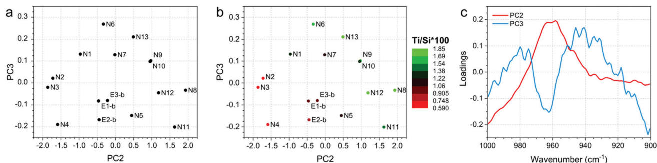
Fig. 4 (a) PC2 and PC3 scores plot, (b) PC2 and PC3 scores plot, in which the sample spots were scaled according to the Ti/Si \times 100 and (c) loadings plot of the PCA model developed on ATR-IR data.
