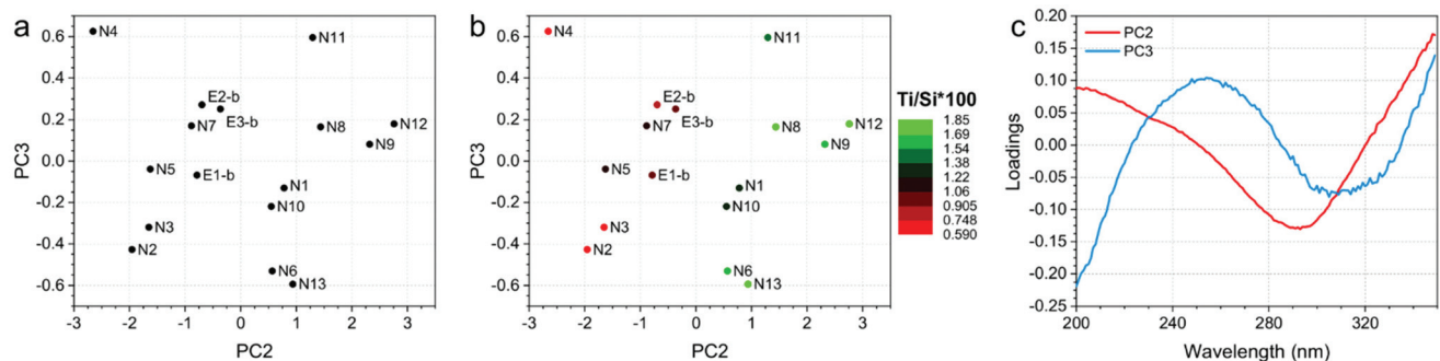
Fig. 5 (a) PC2 and PC3 scores plot, (b) PC2 and PC3 scores plot, in which the sample spots were scaled according to the Ti/Si \times 100 and (c) loadings plots of the PCA model developed on DR-UV data.
