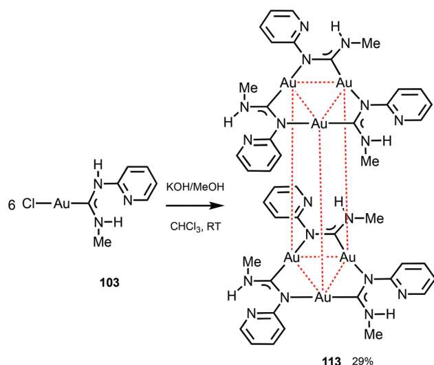
Scheme 17 Generation of 113 and pairwise association through Au...Au interactions (dotted red lines). Au...Au separations are 3.2532(9) Å (intramolecular contacts) and 3.2644(12) Å (intermolecular contacts). 29
