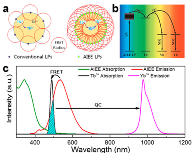
Fig. 7 (a) Schematic illustration of the difference between conventional emission and AIEE in the sensitization of quantum cutting. (b) Energy-transfer pathway from the AIEE LPs to NPs. (c) Normalized absorption and photoluminescence spectra of the AIEE dye and NPs. Reprinted with permission from ref. 125. Copyright (2018) American Chemical Society.
