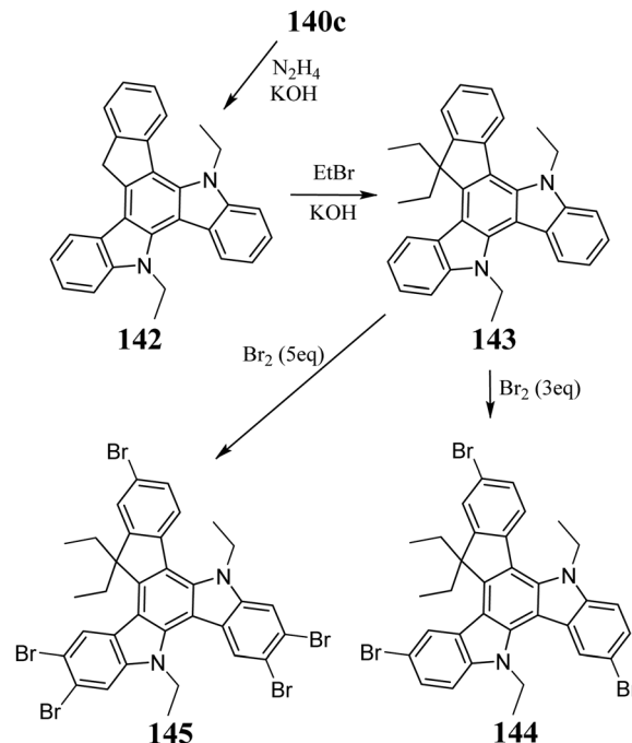
Scheme 47 Synthesis and reactivity of 5,10-diazatruxene.
