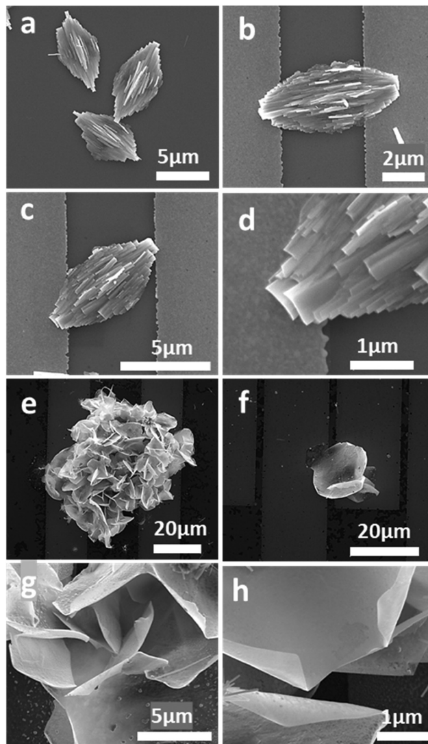
Fig. 3 SEM image of (a) several ZNLs, (b) and (c) a single ZNL connecting two gold electrodes, (d) at high magnification of a single ZNL, (e–h) SEM images at different magnifications of ZNLs.
