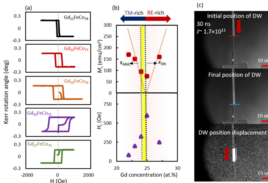
Fig. 1 (a) MOKE measurements as a function of perpendicular magnetic field for Gd_xFeCo_{100-x} films at room temperature. (b) Saturation magnetization and coercivity as a function of Gd composition. (c) Configuration of domain wall (DW) motion in Gd_xFeCo_{100-x} wire with consecutive current pulses. A large external magnetic field along the out-of-plane was applied to saturate the magnetization and generate an up-down and/or down-up DW to initiate DW propagation from the large contact pad area. The position of DW was displaced before and after applying a pulse current. Red and blue dotted lines show the initial and the final position of DWs in the PMOKE image. The DW motion took place in the direction of the injected current.
