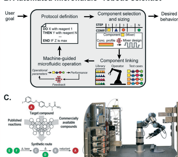
Fig. 5 Outlook for machine learning in microfluidics. (A) To effectively learn microfluidic performance across the field, community repositories are needed consisting of standardized designs, fabrication protocols, and performance metrics together with predictive models previously trained on standardized datasets. These datasets and models can be retrieved by researchers, and adapted to new applications through transfer learning with additional smaller datasets. Sharing the updated models on community repositories completes a positive feedback cycle to continuously extend the predictive understanding of microfluidics to new components and applications. (B) Once the performance of enough components are accurately predicted, they can be integrated into an ML-guided “robot scientist” that can route together different components for fully-automated hypothesis testing and optimization. (C) Such a system has been successfully implemented in automated synthesis of organic compounds using millifluidic flow modules. From Coley et al. , 2019. 113 Reprinted with permission from AAAS.
