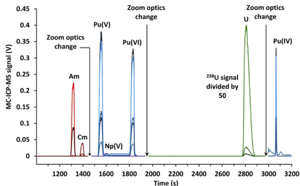
Fig. 6 Electropherogram obtained by CE-MC-ICP-MS for actinides in a spent MOX fuel sample with a 120 mmol L -1 \alpha -HMBA electrolyte. The line breaks were caused by the change in zoom optics during the CE separation.
