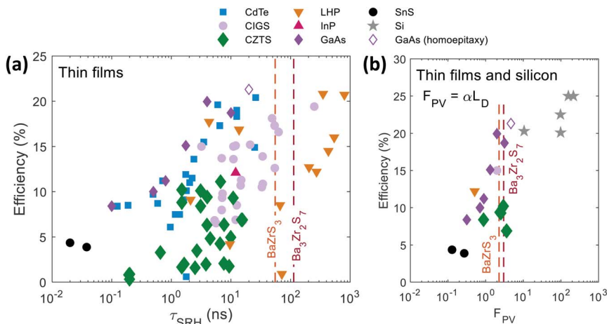
Fig. 6 SRH lifetime ( \tau_{\text{SRH}} ) and solar cell figure of merit F_{\text{PV}} = \alpha L_D vs. energy conversion efficiency for various photovoltaic materials. \text{BaZrS}_3 and \text{Ba}_3\text{Zr}_2\text{S}_7 are plotted as dashed lines corresponding to the best-estimates of our TRPL data analysis; no solar cells of either material have yet been reported. In (a), we only show data for which \tau_{\text{SRH}} and device measurements were performed on samples that were synthesized in the same laboratory and using as close to the same procedure as is reasonably possible; in (b), we additionally require that D and \alpha are reported on comparable samples, with the exception of silicon and GaAs for which we use tabulated values. Data are adapted from ref. 28 and 30–32.
