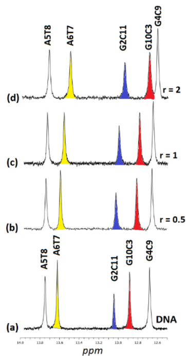
Fig. 9 Part of the 1 H NMR spectra of the d(5'-CGCGAATTCGCG-3') 2 (a) free, and upon addition of (5)Cl 4 at r = 0.5, 1 and 2, (b–d), showing the imino protons of the W.–C. hydrogen bonds.
