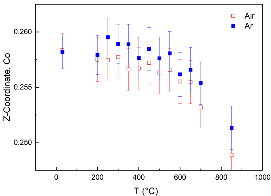
Fig. 16 Z-coordinate of Co in BGLC ( x = 0, y = 0.2 ) upon heating from RT to 850 °C in air and Ar atmosphere.
