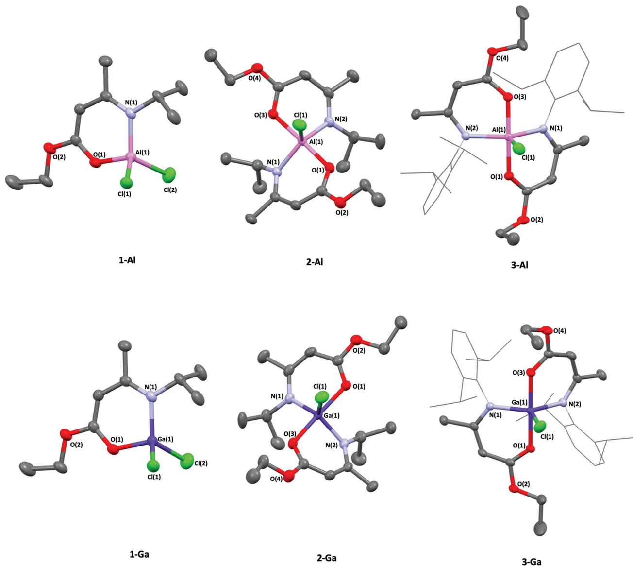
Fig. 3 Molecular structures of aluminium chlorido amidoenoates, [\text{AlCl}_2(\text{AME}^{\text{IPr}})]_2 ( 1-Al ), [\text{AlCl}(\text{AME}^{\text{IPr}})_2] ( 2-Al ), [\text{AlCl}(\text{AME}^{\text{Dip}})_2] ( 3-Al ) and analogous gallium chlorido amidoenoates, [\text{GaCl}_2(\text{AME}^{\text{IPr}})]_2 ( 1-Ga ), [\text{GaCl}(\text{AME}^{\text{IPr}})_2] ( 2-Ga ), [\text{GaCl}(\text{AME}^{\text{Dip}})_2] ( 3-Ga ). Thermal ellipsoids shown at 30% probability. Dip-substituents are shown in wireframe format and hydrogens have been omitted for clarity.
