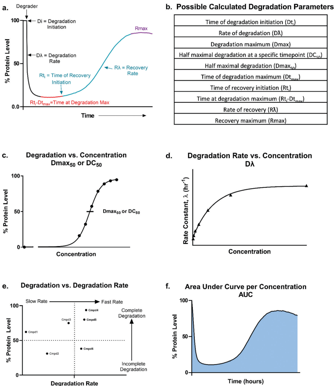
Fig. 2 Overview of degradation profile and quantitative parameters. Model (a) and table (b) outlining the possible parameters which could be generated using the degradation profile. D_{max50} or DC_{50} values (c), degradation rate (d), correlation between percent degradation to degradation rate (e), and area under the curve per concentration (f) can all be calculated or determined from the kinetic degradation profile.
