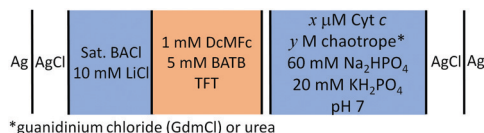
Scheme 1 Schematic of the four-electrode electrochemical cell used for all electrochemical measurements. For blank experiments x was 0\ \mu\text{M} , and with Cyt c in solution x was 10\ \mu\text{M} . For experiments with the chaotropes guanidinium chloride (GdmCl) and urea, y varied from 0 to 12 M. The organic electrolyte salt was bis(triphenylphosphoranylidene)ammonium tetrakis(pentafluorophenyl)borate (BATB). All experiments were carried out under aerobic conditions.
