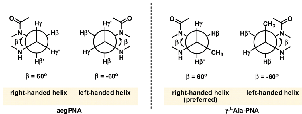
Fig. 8 The gauche conformation of the N(H)–C \gamma –C \beta –N(CO) groups necessitates pre-organization into the right-handed helix in \gamma -(S)-methyl PNA. The structure is viewed along the C \gamma –C \beta axis (adapted with permission from ref. 42. Copyright 2006 American Chemical Society).
