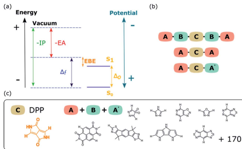
Fig. 1 (a) Definition of -IP , -EA , \Delta_0 , \Delta_f , and EBE , (b) composition of the different dyes studied in terms of their building block with an example ABCBA dye and (c) dye building blocks (explicitly shown hydrogen atoms, other than those connected to nitrogen atoms, indicate carbon atoms where building blocks can be connected to other building blocks in the dyes).
