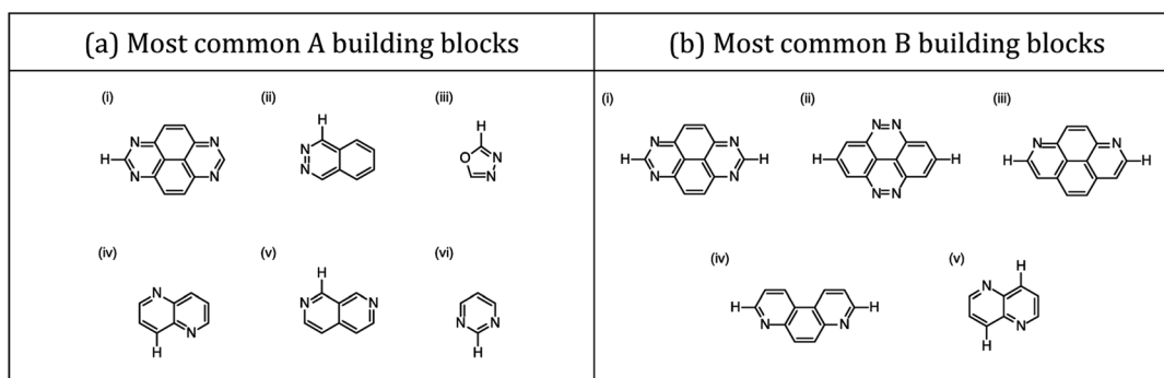
Fig. 11 Most common building blocks on (a) the A and (b) B sites for the ABCBA dyes in the dye-sensitized proton reduction region (explicitly shown hydrogen atoms, other than those connected to nitrogen atoms, indicate carbon atoms where building blocks can be connected to other building blocks in the dyes).
