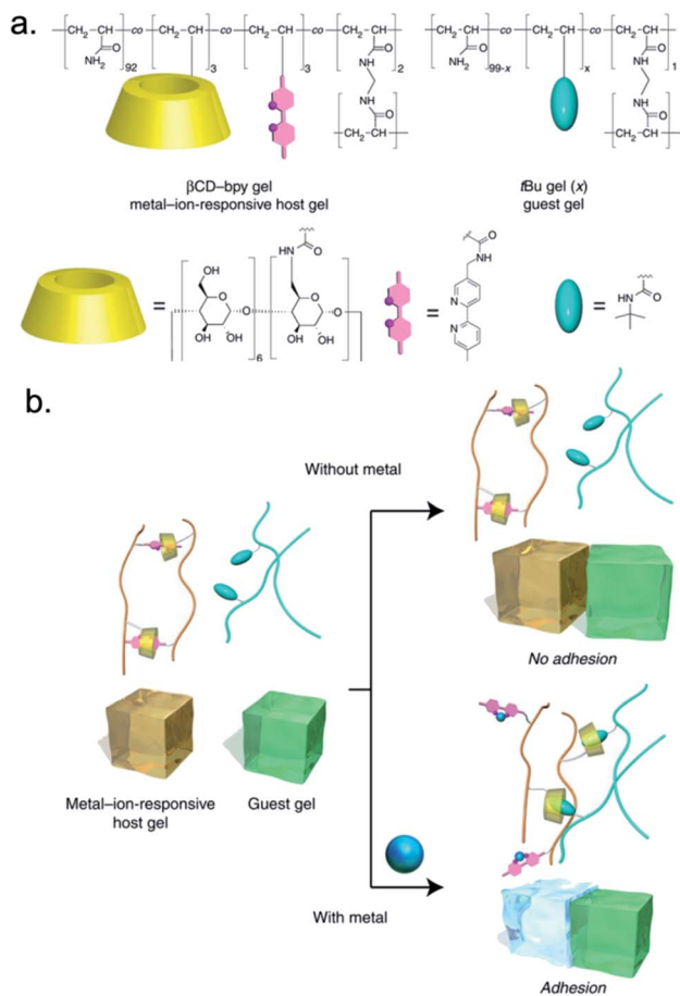
Fig. 10 Metal-ion mediated interfacial adhesion based on host-guest interactions between two hydrogels. (a) Structures of \beta CD-BIPY hydrogel and N - t -BuAAm hydrogel. (b) Metal ion modulates adhesion by forming new host-guest interaction between \beta CD-BIPY hydrogel and N - t -BuAAm hydrogel. Adapted from ref. 68. Copyright 2014 Springer Nature ( http://creativecommons.org/licenses/by/4.0/ ). 68
