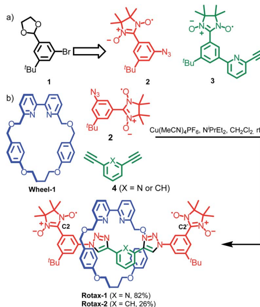
Scheme 1 (a) Protected 3-bromo-5- t -Bu-benzaldehyde starting material used in the synthesis of nitronyl nitroxide based half-axles 2 and 3 (used in the synthesis of Rotax-3 , vide infra ). (b) Synthesis of spin-labelled rotaxanes Rotax-1 and Rotax-2 . The structures of corresponding axles, Axle-1 and Axle-2 are identical with the omission of the macrocycle.
