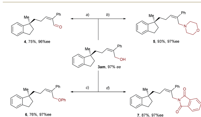
Scheme 3 Derivatizations of the aryl-allylation product.
