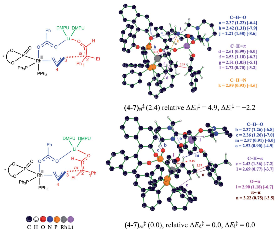
Fig. 3 Optimized transition state geometries for the enantioselective C-C bond formation between the Li-enolate ( 6 2 ) and Rh- \pi -allyl intermediate ( 4 ). Important interatomic distances (in Å) and the corresponding electron densities ( \rho \times 10^{-2} ) at the bond critical points are shown in parentheses along with the strength of the respective noncovalent interactions (in kcal mol -1 ) in square brackets. The relative Gibbs free energies with respect to the lowest energy transition state are in kcal mol -1 .
