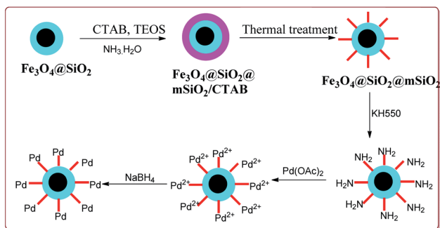
Scheme 9 Preparation of immobilized \text{Fe}_3\text{O}_4@SiO_2@mSiO_2\text{-Pd}(0) nanocatalyst.
