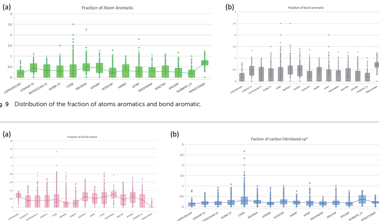
Fig. 10 Distribution of the fraction of chiral carbon and fraction carbons hybridized sp^3 .
