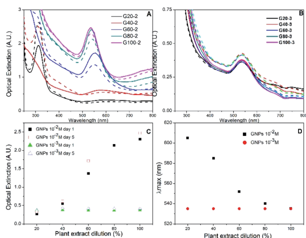
Fig. 1 UV-Vis absorption spectra of GNPs synthesized with different extract dilutions for HAuCl 4 concentration of 1 × 10 -2 M (panel A) and 1 × 10 -3 M (panel B), collected on day 1 (dashed lines) and day 5 (continuous lines). The maximum optical extinction and the plasmon band location as function of extract dilution are shown in panels (C) and (D) respectively.
