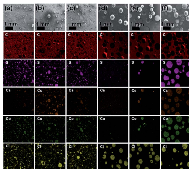
Fig. 2 SEM-EDS elemental mapping of the polymer waste forms for C, S, Cs, Co, and Cl elements: (a–c) represent the elemental mapping for BG polymer waste form top, middle, and bottom sections, respectively; (d–f) display the elemental mapping for NG polymer waste form top, middle, and bottom sections, respectively.
