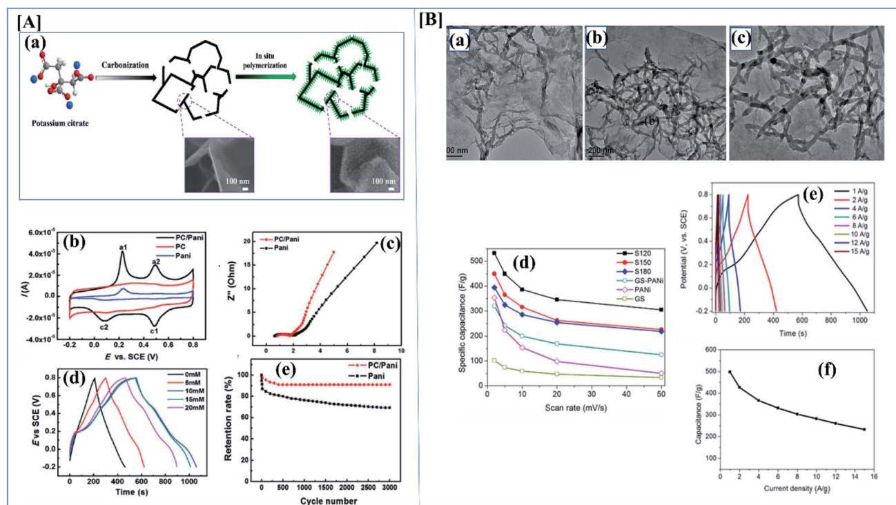
Fig. 10 [A] (a) Synthesis route for PC/PANI composite. (b) CV curves of the electrodes of PC/PANI composites, PC, and PANI at 0.05 \text{ V s}^{-1} . (c) Nyquist plots of PC/PANI composite. (d) GCD curves of PC/PANI composites with different concentrations of aniline at 1.0 \text{ A g}^{-1} . (e) Cycle stability of composites at a constant current density of 5.0 \text{ A g}^{-1} (reprinted with permission, 104 copyright 2018 Wiley) [B] (a–c) TEM images of GO/PANI composites at different temperatures of 120, 150 and 180 °C. (d) Specific capacitance of GNS/PANI composites at different scan rates. (e) The GCD curves with different current densities of GO/PANI composites synthesized at 120 °C. (f) Specific capacitance of GO/PANI composites at different current densities (DOI: 10.1038/srep44562, Open source Nature).
