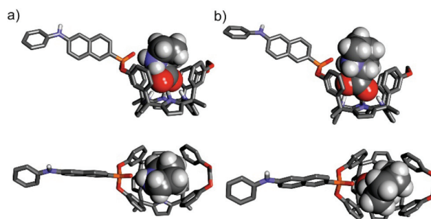
Fig. 10 Side and top views of the energy-minimized inclusion complexes L-ProC1in (a) and L-PipeqC1in (b). The structures are energy minima at the BP86/def2-SVP level of theory. The receptors are shown in stick representation. Non-polar hydrogen atoms were removed for clarity. The included amino acids are depicted as CPK models.
