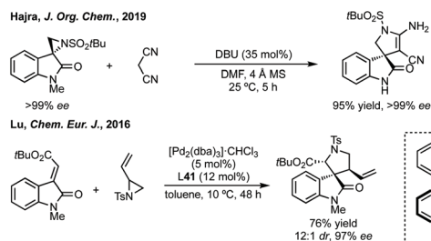
Scheme 41 3,3'-Spiropyrrolidine oxindoles synthesised by aziridine ring expansion.
