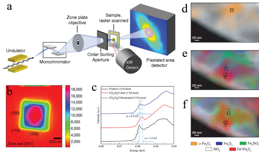
Fig. 7 (a) STXM and SXFM setup; Copyright 2014, National Academy of Sciences; (b) SXFM image of a \text{Cu}_2\text{O} nanoparticle; Copyright 2019, Springer Nature; (c) scanning X-ray nanospectroscopy of the (110) facet; Copyright 2019, Springer Nature; (d) to (f) chemical contour images of the catalyst under different treatments; Copyright 2008, Springer Nature. All panels reproduced with permission. 148,156,160
