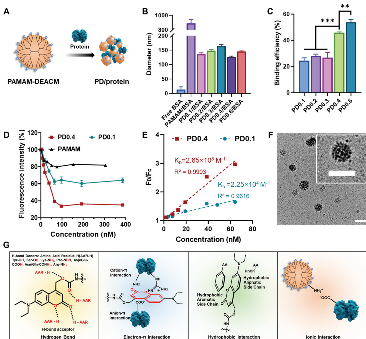
Fig. 1 DEACM-modified dendrimer binds to protein. (A) Schematic illustration of the co-assembled PD/protein nanocomplex. (B) DLS results of free BSA, PAMAM/BSA mixture and PD/BSA nanocomplexes. (C) Protein binding efficiency of a series of PAMAM–DEACM. (D) Fluorescence change of rBSA (100 nM) with different concentrations of PAMAM–DEACM or PAMAM. (E) The Stern–Volmer curve for the interaction of PAMAM–DEACM with rBSA (100 nM). F_0 is the fluorescence intensity of rBSA, F_c is the fluorescence intensity of PD/rBSA. \lambda_{ex} = 548 nm, \lambda_{em} = 586 nm. (F) TEM images of PD0.4/BSA. Scale bar: 200 nm. (G) Possible interactions between PAMAM–DEACM and proteins: hydrogen bond, electron– \pi interaction, hydrophobic interaction, and ionic interaction. Data analysis: n = 3, *** p < 0.001, ** p < 0.01.
