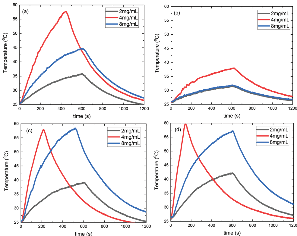
Fig. 9 Experimental curves of heating sequence during MH of (a) S_1@Pt , (b) S_2@Pt , (c) S_3@Pt and (d) S_4@Pt at three different concentration values namely 2, 4 and 8 mg mL -1 . AMF amplitude and frequency were set to 24 kA m -1 and 765 kHz respectively. The concentration value of 4 mg mL -1 presented the higher heating rate verifying theoretical estimations.
