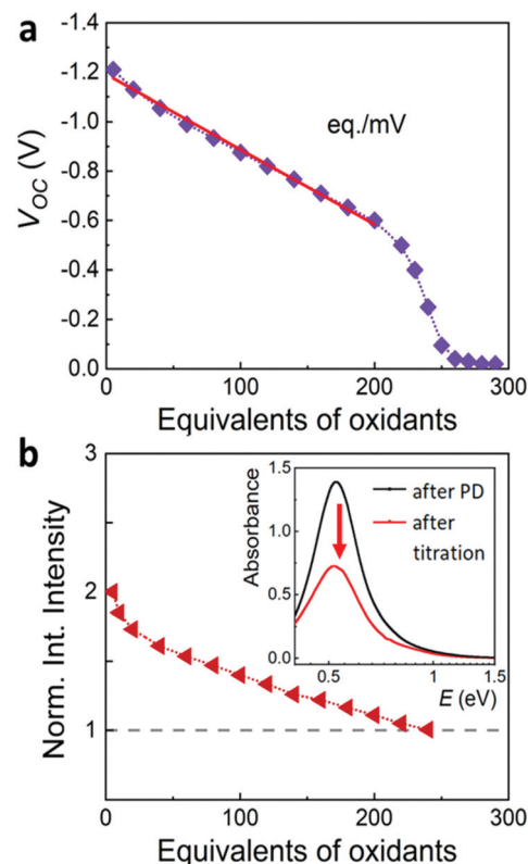
Fig. 2 (a) Illustration of a typical monitoring of the open circuit voltage ( V ) in an electrochemical cell upon potentiometric titration by introducing oxidants in the solution. From the slope of this plot it is possible to extract capacitance values with C = \Delta q/\Delta V , where the number of charges q is determined by the oxidant added. (b) Illustration of a typical normalized integrated intensity of the plasmonic resonance (LSPR) as a function of the equivalents of oxidants added until full recovery of the initial optical properties. Inset shows the decrease in the intensity of the plasmonic resonance upon addition of increasing equivalents of oxidants (red arrow). 32
