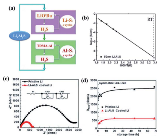
Fig. 14 (a) Schematic illustration of \text{Li}_x\text{Al}_y\text{S}_z ALD, (b) Arrhenius plot for temperature-dependent ionic conductivity measured using a 50 nm \text{Li}_x\text{Al}_y\text{S}_z film, (c) AC impedance spectra of Li/electrolyte/Li symmetric cells using both pristine Li and \text{Li}_x\text{Al}_y\text{S}_z -coated Li after 68 h storage, and (d) R_{\text{SEI}} of Li/electrolyte/Li symmetric cells versus storage time. 40
