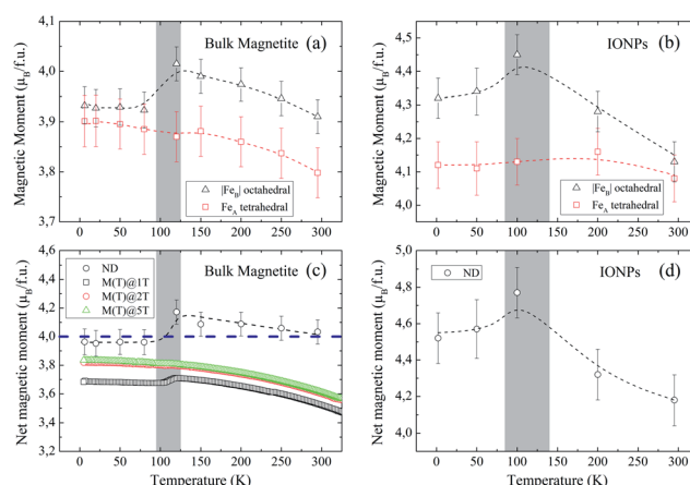
Fig. 5 Thermal variation of the \text{Fe}_{\text{A, B}} magnetic moment for (a) bulk magnetite and (b) IONP samples. Thermal evolution of the net magnetic moment per formula unit (f.u.) for (c) bulk magnetite and (d) IONPs. The blue dashed line corresponds to the theoretical net moment value for stoichiometric magnetite. Dashed lines are guides to the eye.
