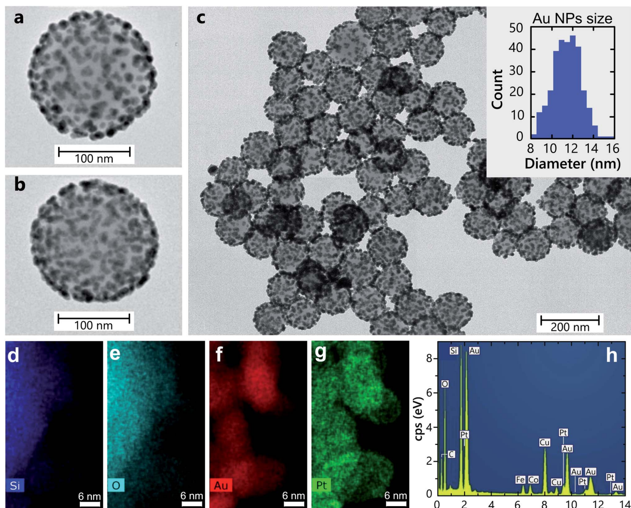
Fig. 1 TEM images of synthesised nanoparticles. (a and b) A single nanoparticle of (a) SiO 2 –Au (3) and (b) SiO 2 –Au (3) –Pt +++ . (c) Statistical analysis of SiO 2 –Au (3) –Pt +++ nanoparticles. Inset shows the size distribution of Au (3) nanoparticles with an average diameter of 12 nm. In order to obtain the images, the solution containing the nanostructures was dried on a TEM grid which led to their partial aggregation. (d–g) High resolution elemental maps and (h) EDS spectrum of SiO 2 –Au (3) –Pt +++ hetero-nanoparticles.
