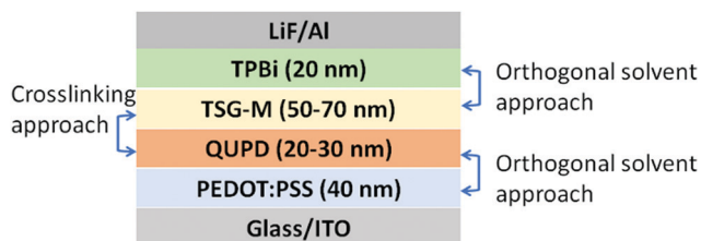
Fig. 16 Schematic of OLEDs structure with four organic layers. QUPD is N,N -bis(4-(6-((3-ethyloxtan-3-yl)methoxy)hexyloxy)phenyl)- N,N -bis(4-methoxyphenyl)biphenyl-4,4-diamine, TSG-M is green emitter. (reproduced from the ref. 95).
