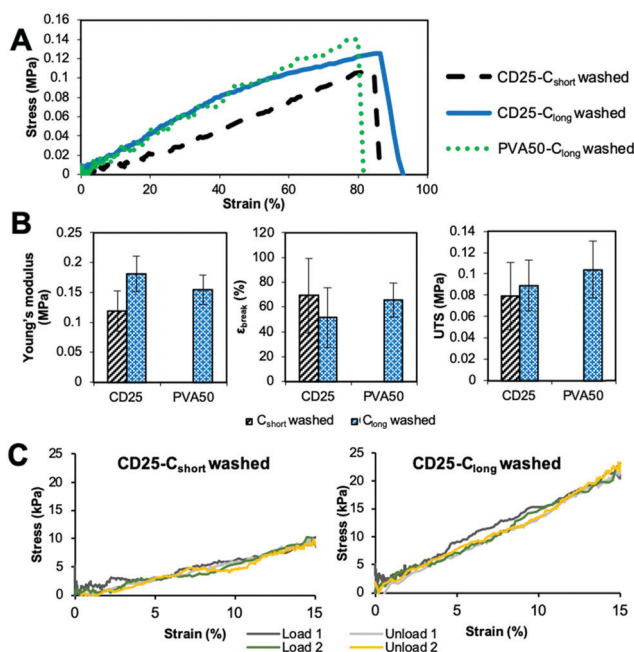
Fig. 8 Mechanical behavior of the scaffolds in the wet state. (A) Typical stress–strain curves, (B) evolution of modulus, strain at break and UTS with curing and washing. The given value is the average value for 3 samples with the standard deviation. (C) Stress–strain curves obtained for cured and washed CD25 samples between 0 and 15% strain.
