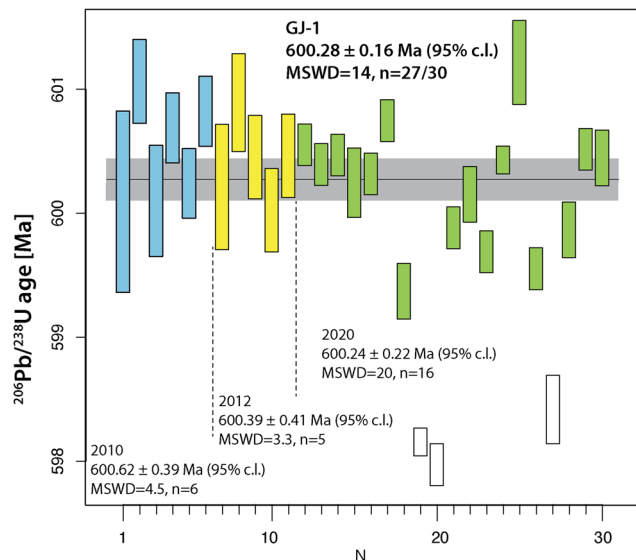
Fig. 6 Compilation of ^{206}\text{Pb}/^{238}\text{U} age determinations of reference zircon GJ-1 at University of Geneva.
