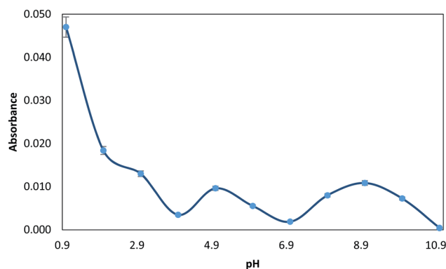
Fig. 2 Effect of pH on the extraction of 10 µg L -1 Hg(II), prepared with 0.01% (v/v) MTS, 0.5% (wt/v) NaCl, and the respective buffer (pH 1–11).
