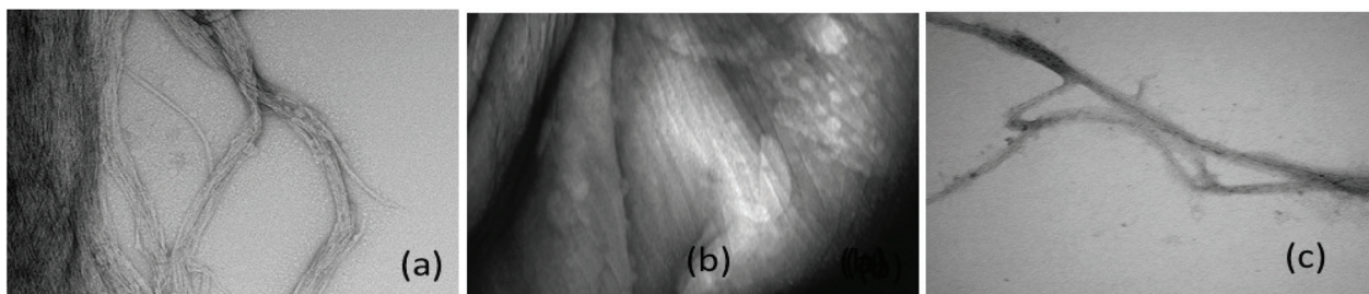
Fig. 9 SEMs after treatment A \beta 42 (5 \mu M) as follows (a) constant agitation 72 hours pH 7.4 @ 37 °C (b) as in (a) including 5 \mu M Zn ^{2+} (c) as in (a) including Zn ^{2+} (5 \mu M) and compound 1 1 \mu M. Bar = 100 nm. Magnification 49 000 \times .
