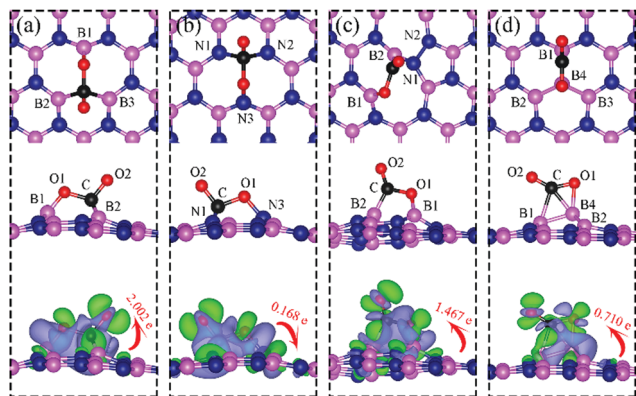
Fig. 13 Top and side views of the most energetically favorable configurations of adsorbed \text{CO}_2 on the dh -BN with (a) \text{V}_\text{N} , (b) \text{V}_\text{B} , (c) SW, and (d) \text{B}_\text{N} . The magenta, blue, black and red balls represent the B, N, C, and O atoms, respectively. The top and middle panel shows the top and side views, respectively. Bottom: The corresponding side views of the geometric structures with the charge density difference plot. The green and violet isosurfaces with iso-value of \pm 0.003 \text{ e} \text{ \AA}^{-3} , represent the accumulation and depletion of electron, respectively. The red arrow shows the electron transfer in direction and value.
