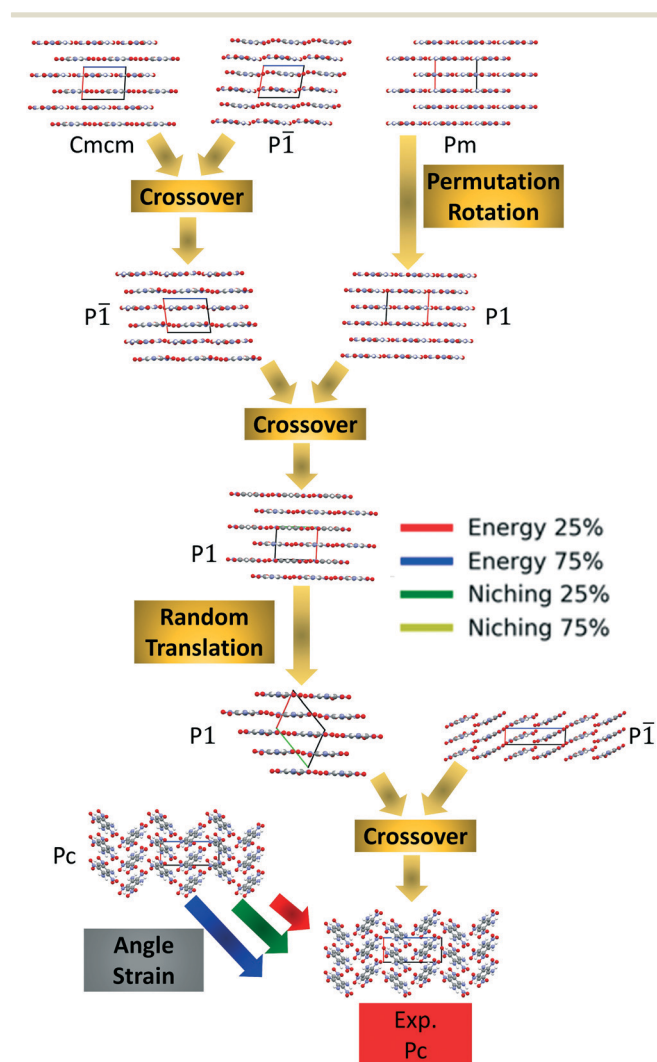
Fig. 11 Evolutionary routes that produced the experimental structure of DATB in different GA runs. The packing motifs and space groups of all structures are shown. The a, b, and c axes are colored in red, green, and blue, respectively.
