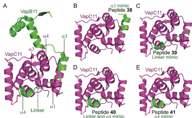
Fig. 11 (A) Crystal structure (6A7V) 149 of the complex between VapB11 (green) and VapC11 (magenta). A representation of the regions selected for the design of VapB11 peptides 38 (helix α3 mimic), 39 (linker mimic), 40 (linker and helix α4 mimic) and 41 (helix α4 mimic) is shown in (B), (C), (D) and (E), respectively.
