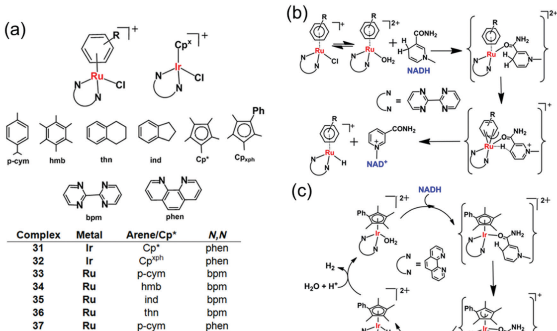
Fig. 11 Cyclopentadienyl Ir III ( 31 , 32 ) and arene Ru II transfer hydrogenation catalysts ( 33 – 37 ) for NADH oxidation. 26 Proposed mechanism for transfer of hydride from 1,4-NADH to (b) Ru II and (c) Ir III complexes involving nicotinamide carbonyl coordination and arene/Cp ring slippage. 26
