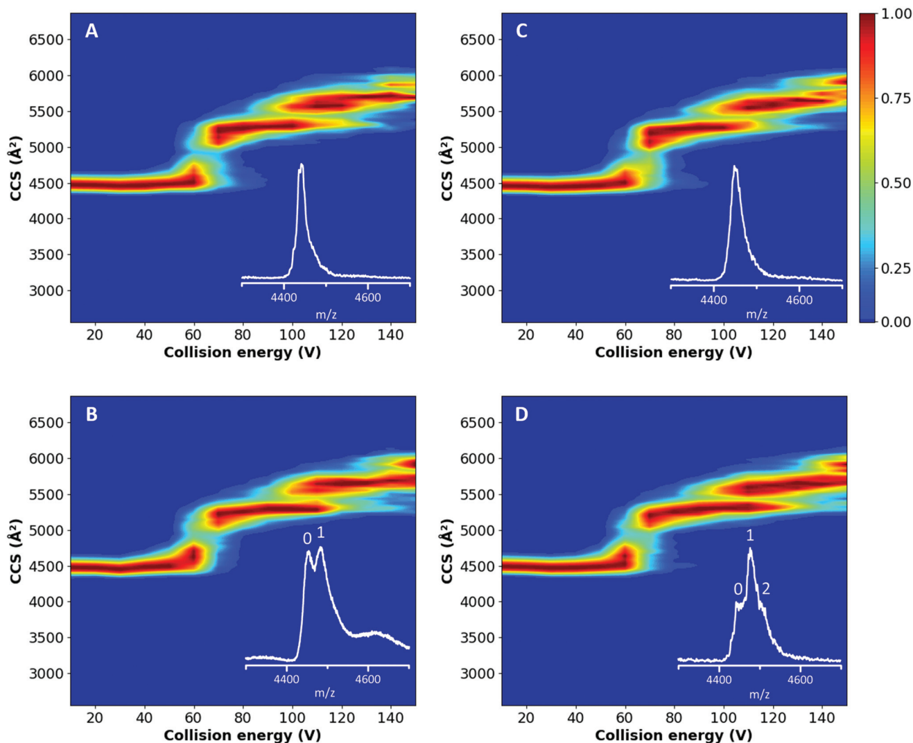
Fig. 3 CIU plots of untreated (A) and delipidated (C) hSA and of the untreated (B) and delipated (D) hSA in complex with PFOA (1:10 protein : PFOA ratio). The ^{TW}CCS_{N_2} is plotted as a function of the trap collision energy and the intensity is shown using a colour scale (red is 100% and blue 0%). The insets show the peaks selected (15+ charge state) for extraction of the ^{TW}CCS_{N_2} at a trap collision energy of 60 V. Arrival times were extracted from the whole peak, including salt adducts and complexes (where appropriate).
